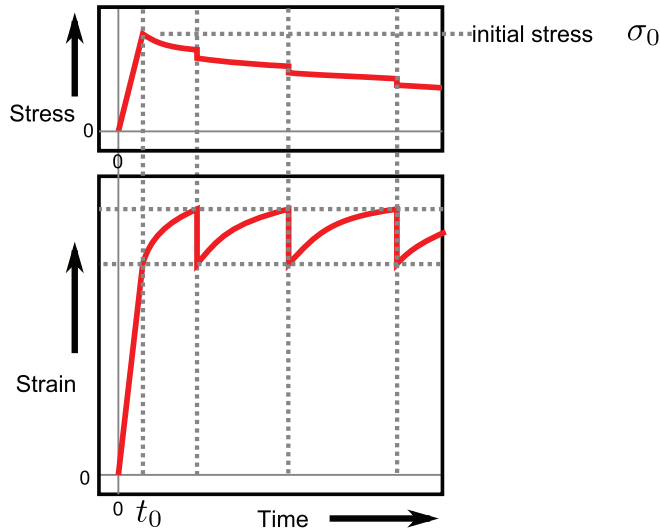
FIG. 2 Typical Relaxation Curves
