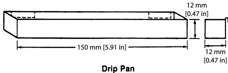
FIG. 4 Heat Release Specimen Holder, Mounting Bracket, and Drip Pan
