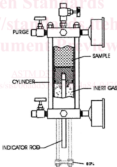
FIG. 1 Typical Floating Piston Cylinder Designs
