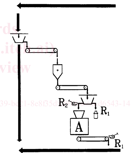
FIG. 3 Analyzer on Secondary Reject—Two-Stage Mechanical Sampling
