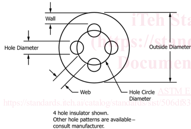
FIG. 1 Wall and Web Thicknesses
