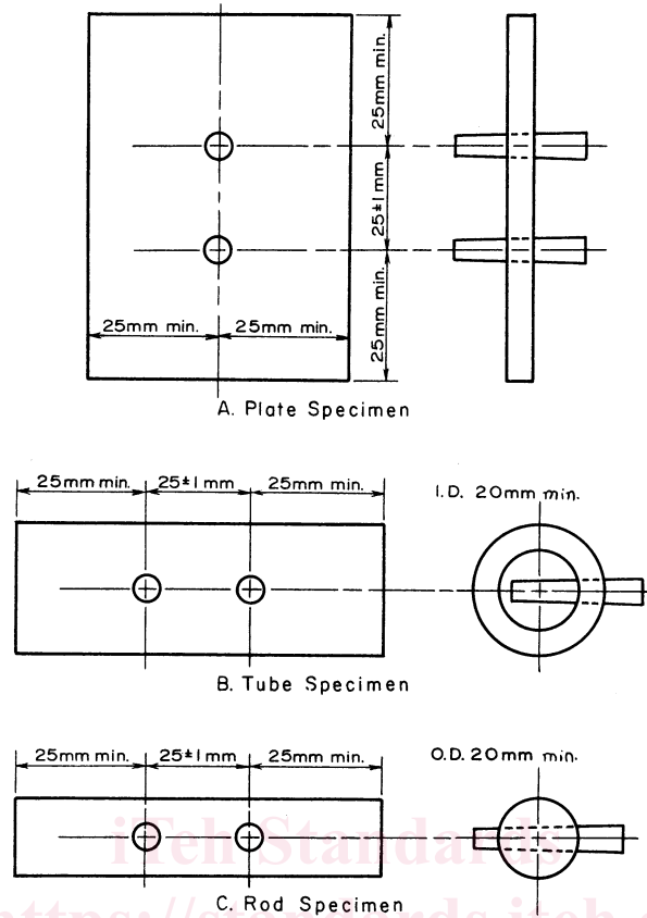
FIG. 2 Taper-Pin Electrodes
