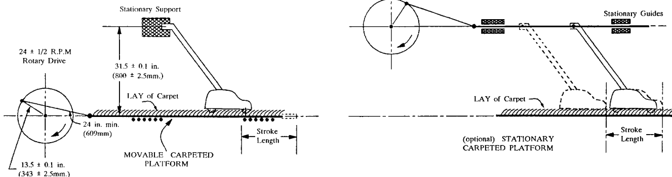
FIG. 1 Test Fixture
