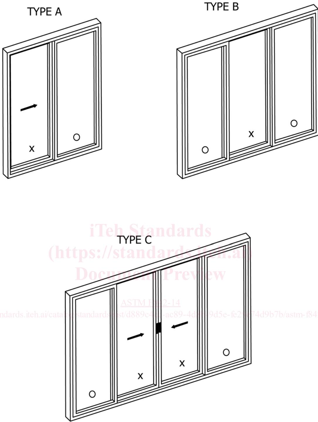
O - Non-operating Door Panel X - Operating Door Panel FIG. 1 Typical Horizontal Sliding Door Assembly Types (viewed from the exterior)
