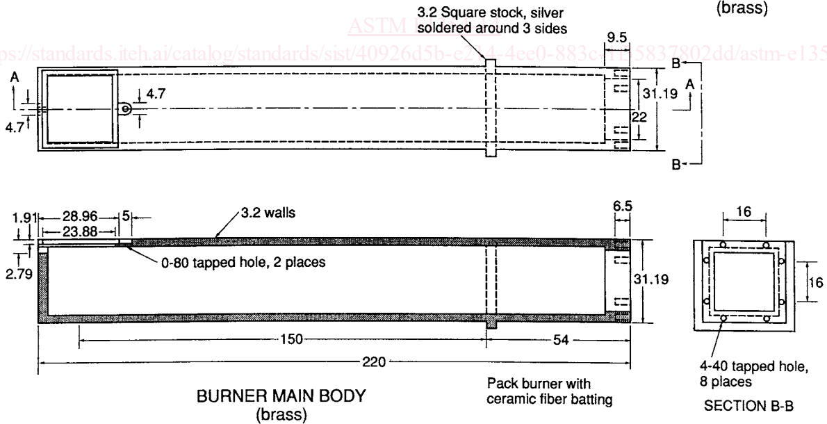
FIG. 11 Calibration Burner
