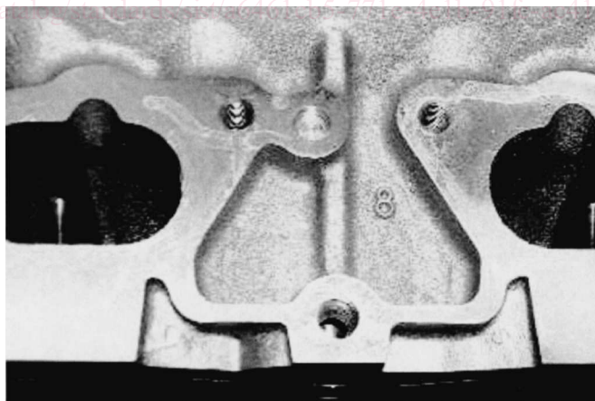
FIG. 7 Cylinder Head
