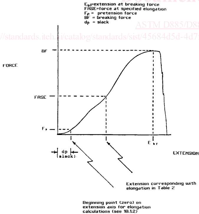
FIG. 1 Force-Extension Curve
