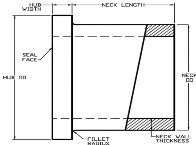
FIG. 1 Polyethylene Flange Adapter Geometry
