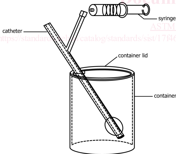
FIG. 3 Balloon Burst Apparatus
