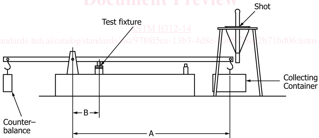
FIG. 2 Transverse Rupture Test Fixture Example of Constant Loading Beam Device
