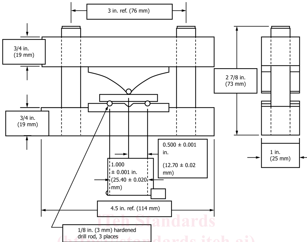
FIG. 1 Example of Constant Loading Beam Device Transverse Rupture Test Fixture
