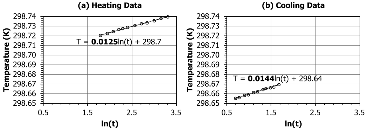
FIG. 42 (a & b) Typical Experimental Test Results
