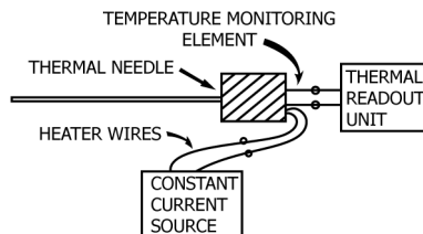
FIG. 1 Thermal Probe Experimental Setup
