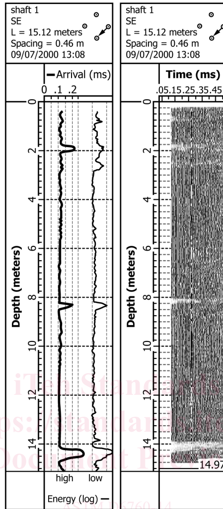
FIG. 2 Typical Ultrasonic Profile
