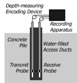
FIG. 3 Test Arrangement
