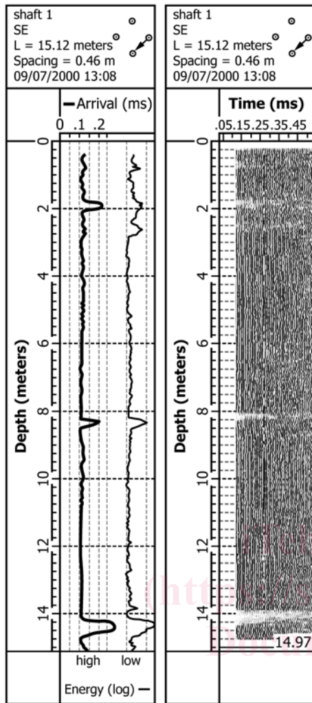
FIG. 2 Typical Ultrasonic Profile
