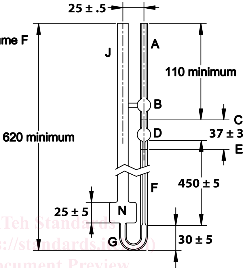
FIG. 1 Cannon Master Viscometer
