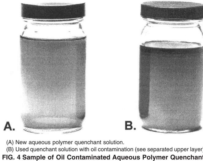
FIG. 4 Sample of Oil Contaminated Aqueous Polymer Quenchant
