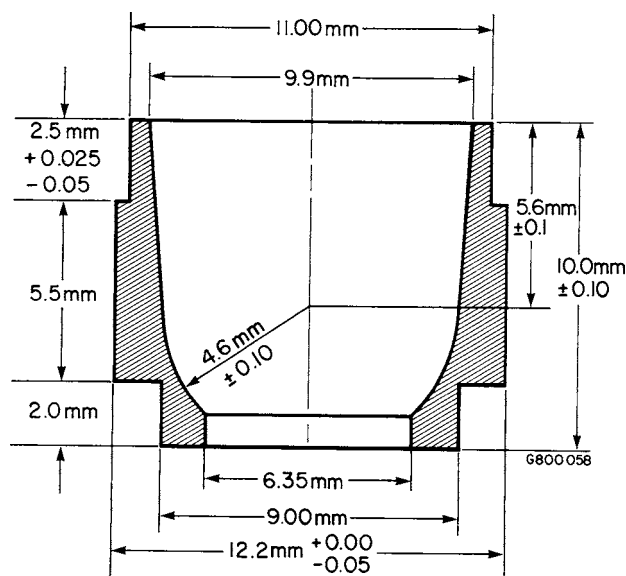
FIG. 2 Sample Cup
