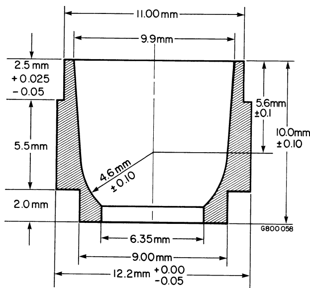
FIG. 2 Sample Cup
