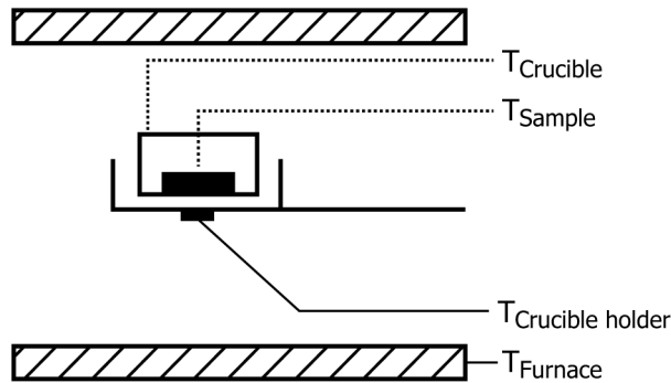
FIG. 12 Magnetic Reference Temperature Sample Positioning for Procedure A
