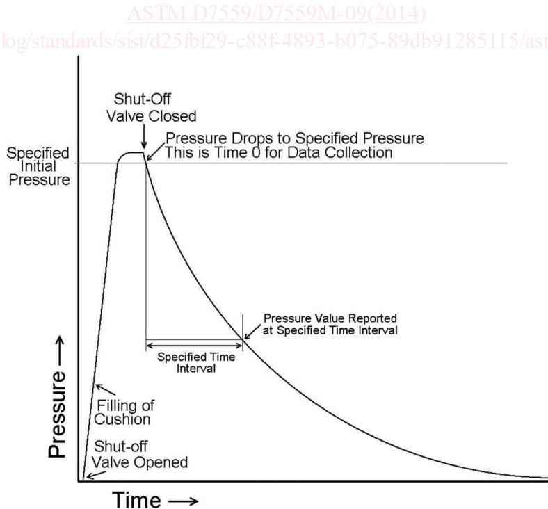
FIG. 1 Test Scheme
