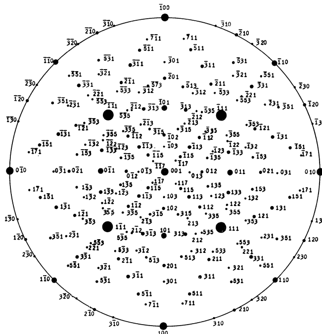
FIG. 4 Polar Chart for Solution of Laue Back Reflection Patterns Standard {001} Projection for a Cubic Crystal
