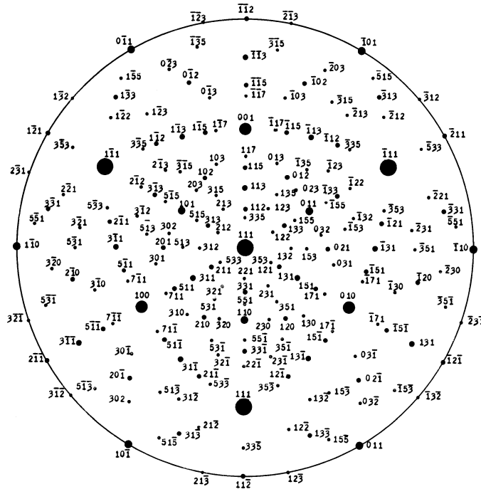
FIG. 5 Standard \{001\}[111] Projection for a Cubic Crystal
