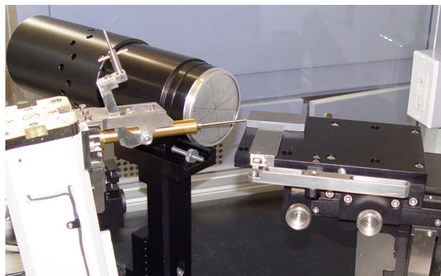
FIG. 2 Universal Camera With Goniometer Head for Back-Reflection Laue Studies Side-Reflection Laue Camera for Turbine Blade Single-Crystal Measurements
