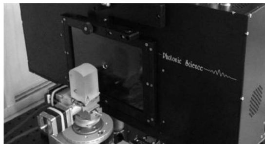
FIG. 1 Back-Reflection Laue Camera for Metallic Sheet Specimens Measuring Sapphire Single Crystal Mounted on a Five-Axis Motorized Goniometer
