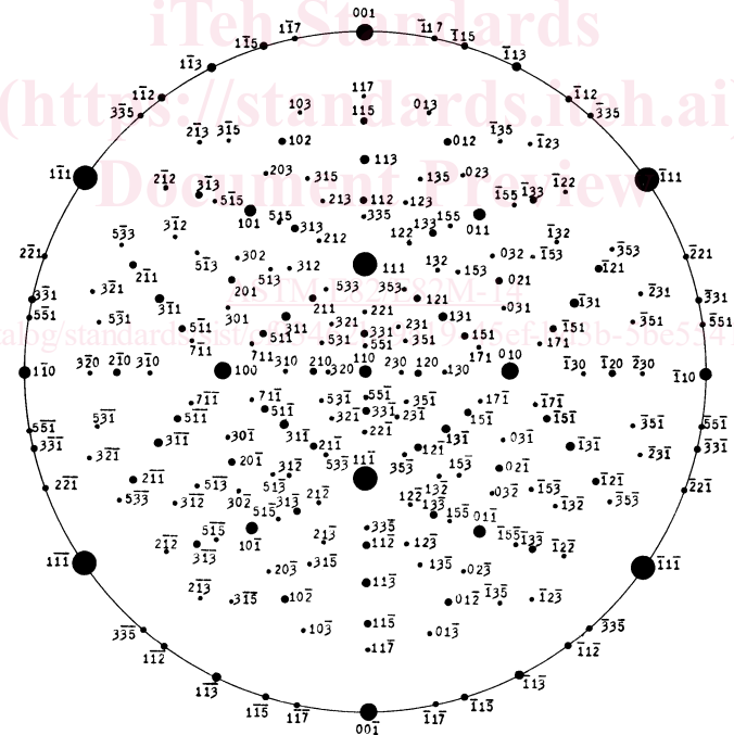
FIG. 6 Standard \{111\}[110] Projection for a Cubic Crystal
