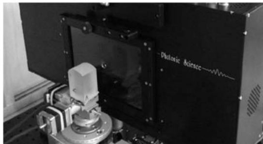
FIG. 1 Back-Reflection Laue Camera Measuring Sapphire Single Crystal Mounted on a Five-Axis Motorized Goniometer
