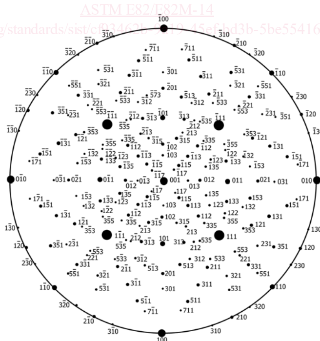
FIG. 4 Standard \{001\} Projection for a Cubic Crystal
