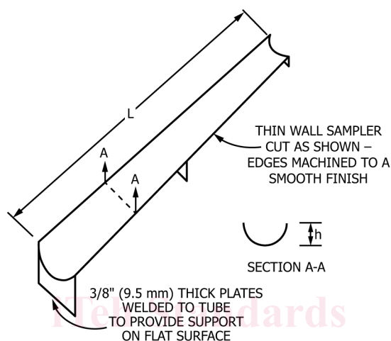
FIG. 1 Example of Soil Slice Trough and Holder
