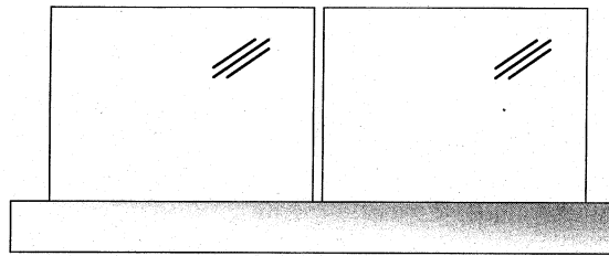
FIG. 7 Type V: One-side Support with Protective Top One-Side Support—Glazing as Structural Member Rail—Structural
