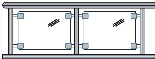
FIG. 5 Type IV: Three-side Support—Structural Edge Clamping Glazing System—Glazing as Infill
