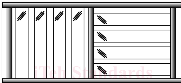
FIG. 3 Type II: Two-side Support—Multiple Lite Glazing as Infill
