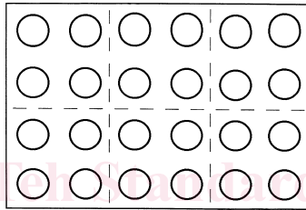
FIG. 6 Patty Positions for Heavy-Load Tests on a 3 by 2-ft (0.6 by 0.9-m) Griddle Surface
