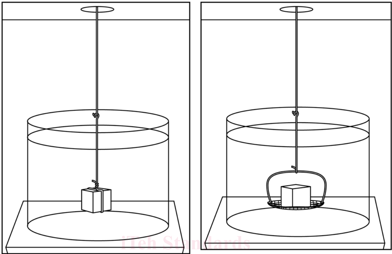
(a) Twisted wire arrangement (b) Basket support arrangement FIG. 1 Methods for Holding the Test Specimen When Weighing in Water
