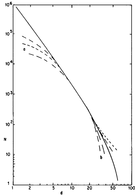
\Sigma N = cumulative number of particles per unit mass of powder d = particle diameter (see 5.1) The solid line represents the “real” count. The broken lines represent failures to obtain correct counts because of either presenting too many particles to the counter, a, or of presenting too few, b.
