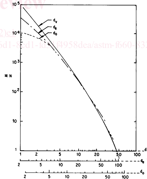
\Sigma N = cumulative number of particles per unit mass of powder d = particle diameter, \mu\text{m} (see 5.1)
