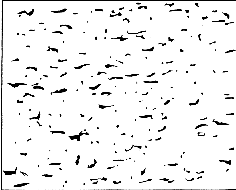
FIG. 4 — 5.0 % Porosity
