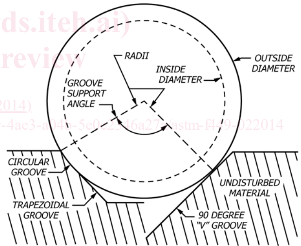
FIG. 2 Support Grooves
