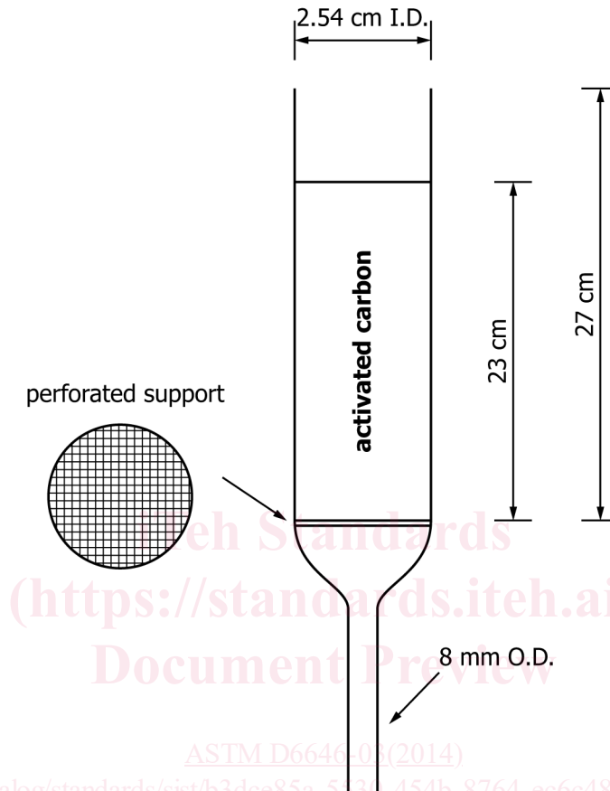
FIG. 1 Schematic of Adsorption Tube
