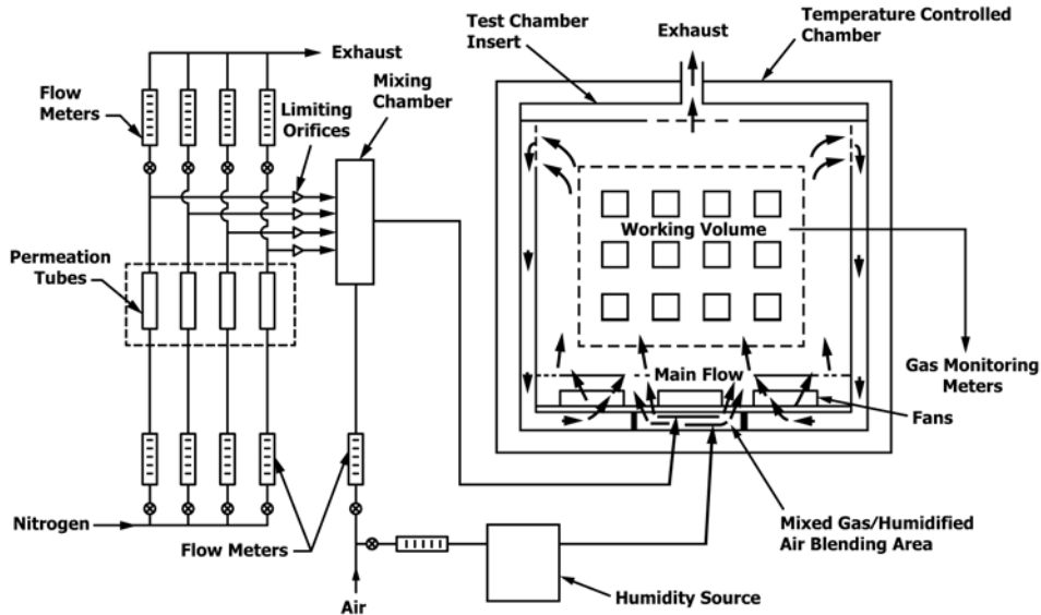
FIG. 2 Schematic Vertical Recirculating Mixed Flowing Gas (MFG) Test System
