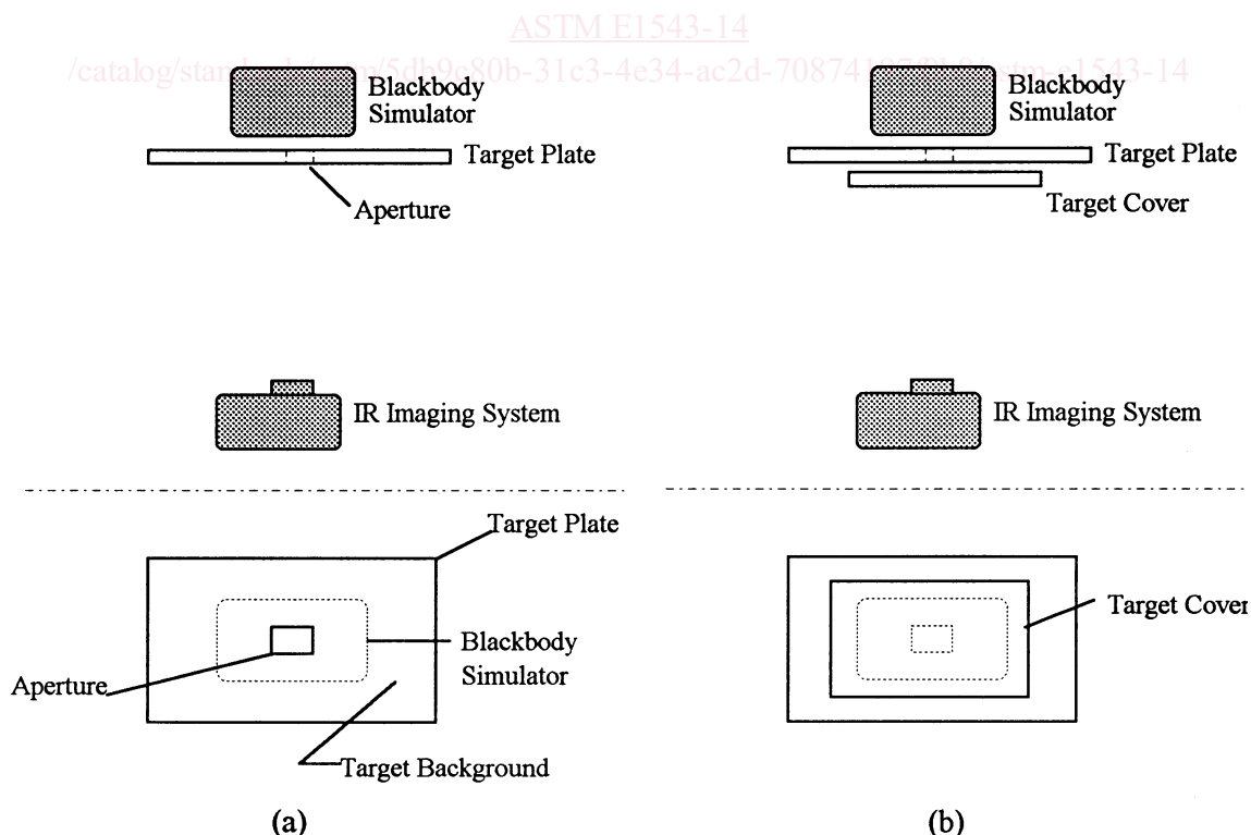
FIG. 1 Schematic of NETD Test Procedure Configuration; (a) When Measuring Signal and (b) When Measuring Noise
