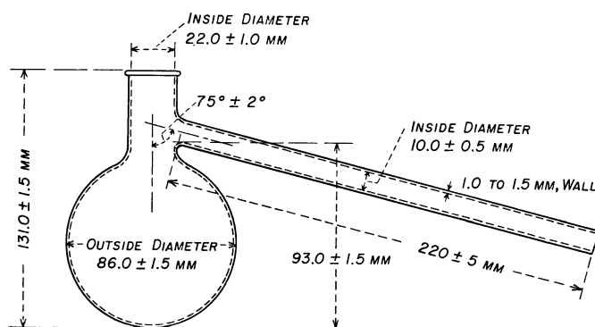
FIG. 1 Distillation Flask
