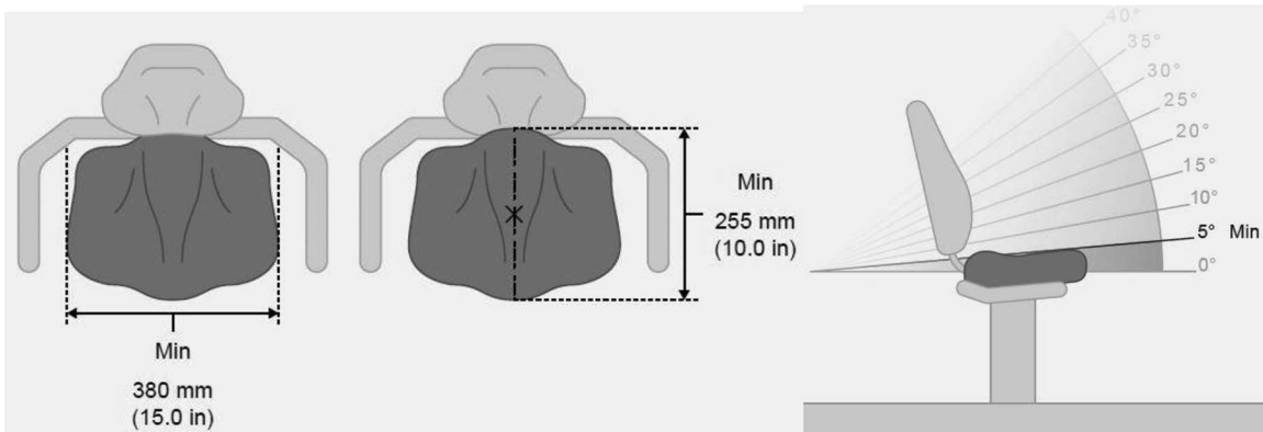
FIG. 4 Minimum Seat Dimensions – Width, Depth, Angle
