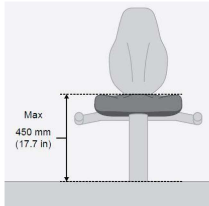
FIG. 5 MinimumMaximum Seat Dimensions – Height
