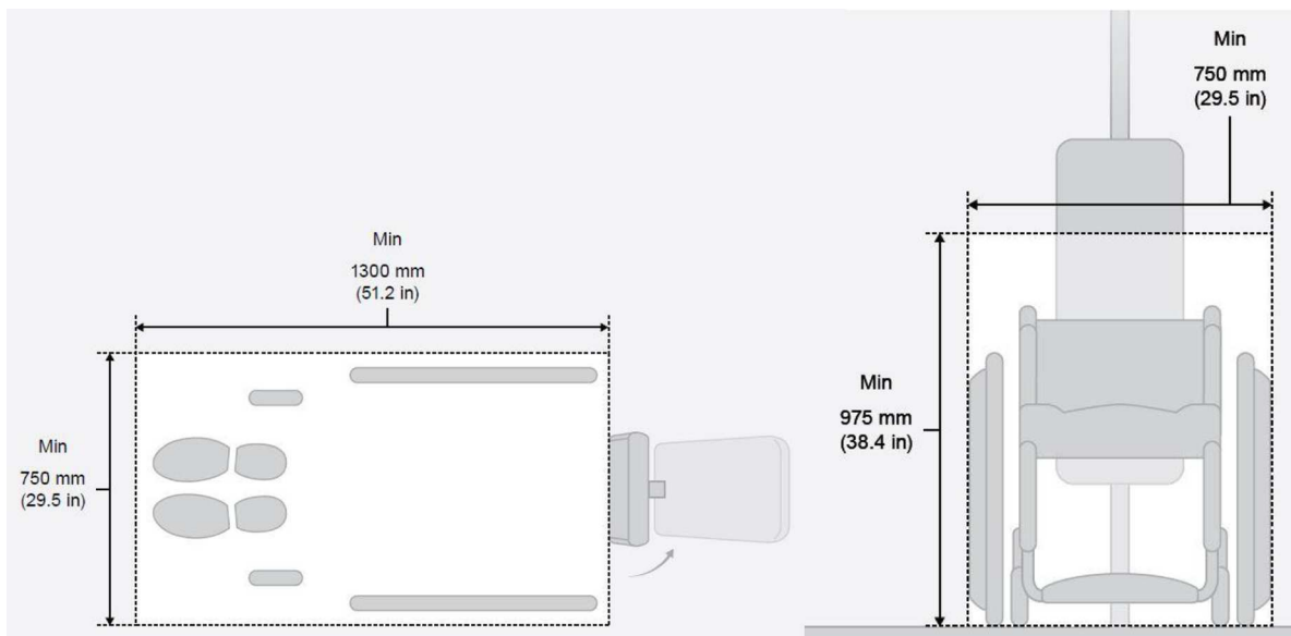
FIG. 6 Removable/Movable Minimum Clear Space Area
