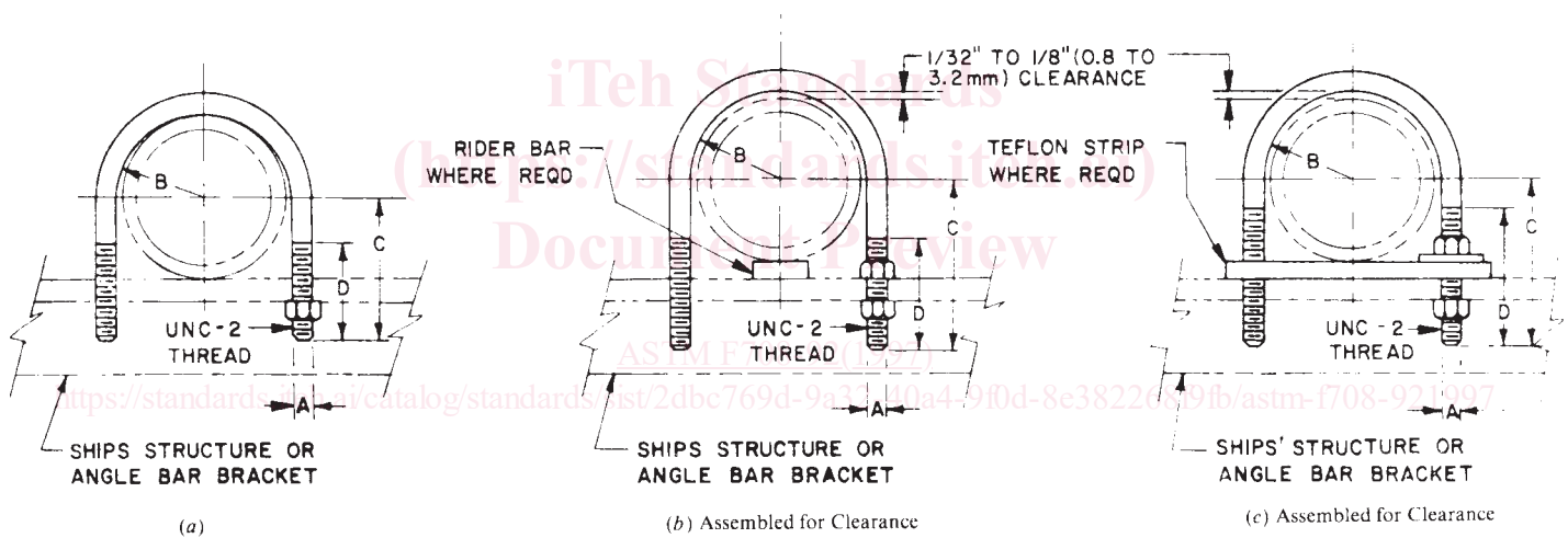
FIG. 3 Welded Hangers
