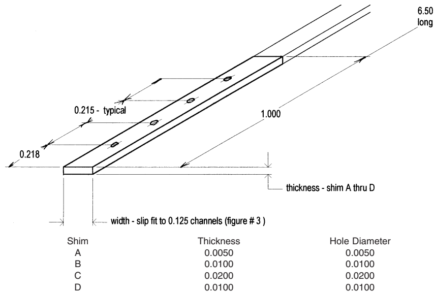
FIG. 4 Shims
