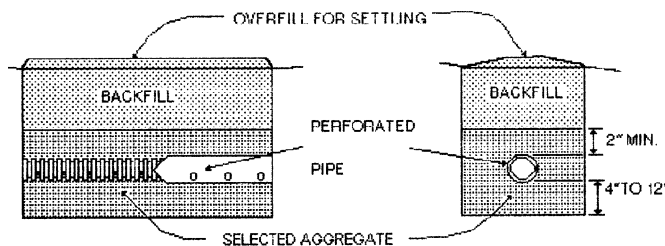
FIG. 1 Gravel Leach Trench
