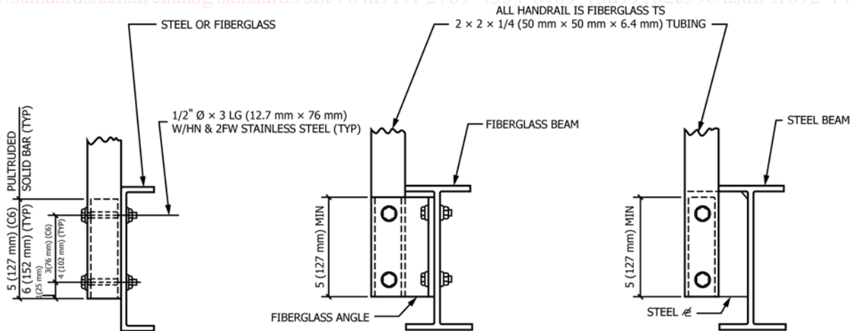
FIG. 3 Pedestal/Stanchion Mount NOTE 1—All joints to be epoxied and bolted or riveted.
