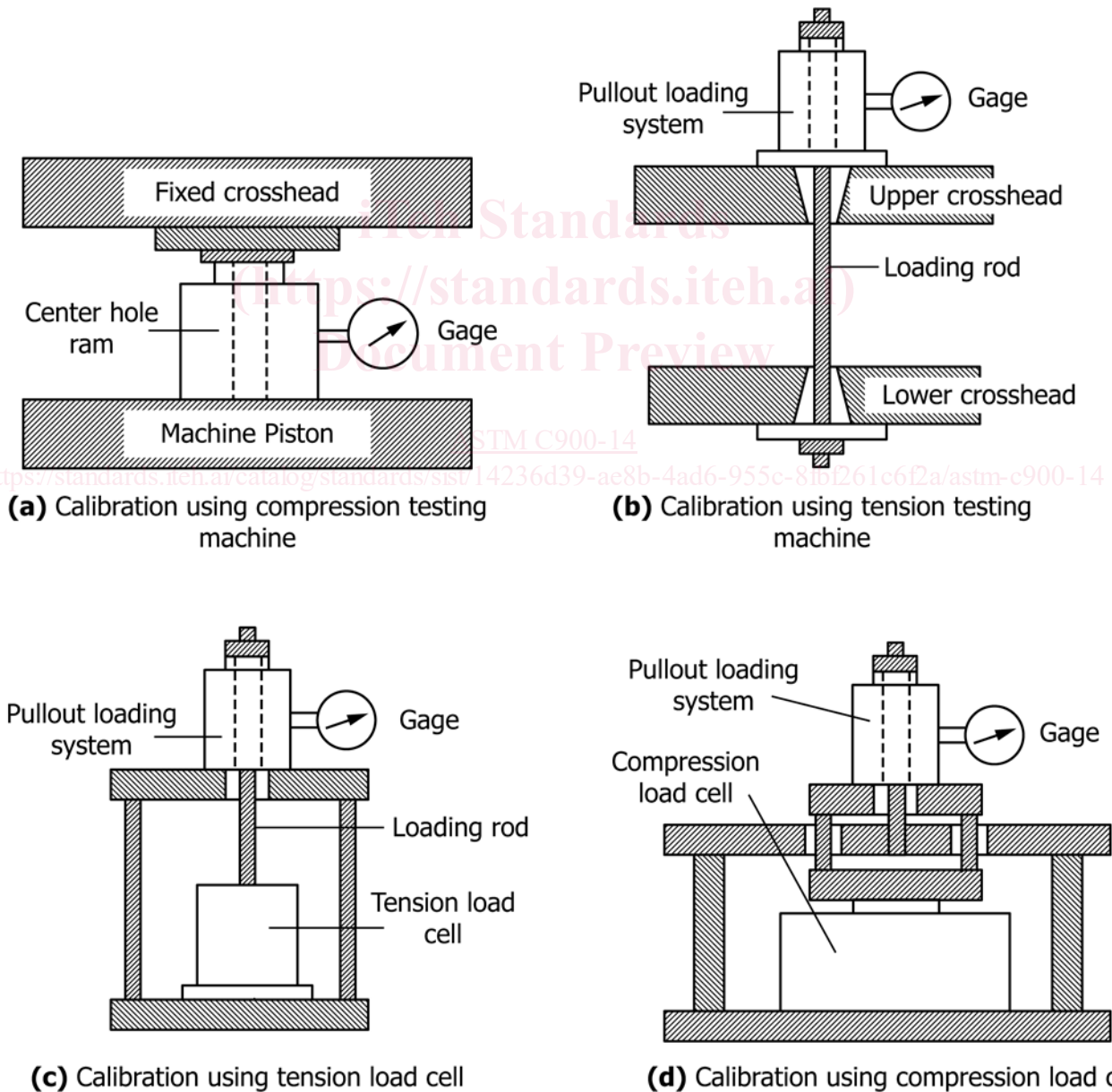
FIG. A1.1 Schematics of Acceptable Methods to Standardize Pullout Load Measuring System
