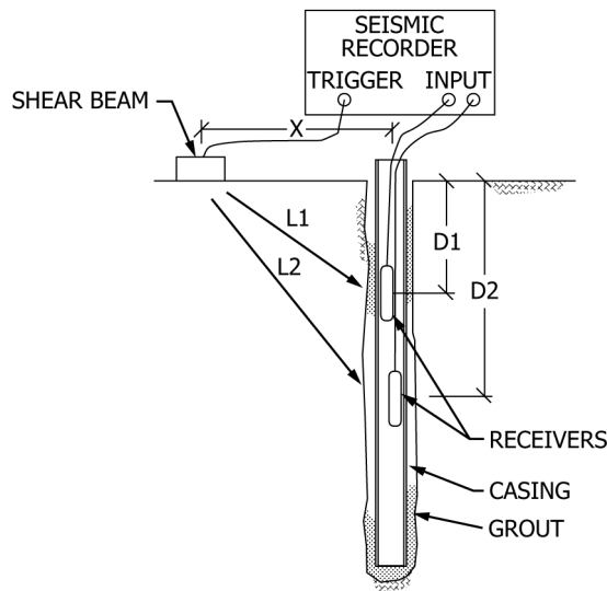
CROSS-SECTION VIEW
