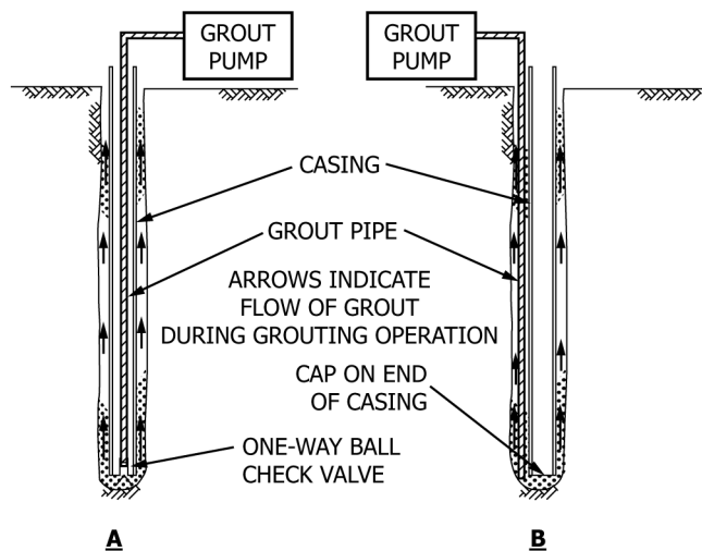
CROSS-SECTION VIEW
