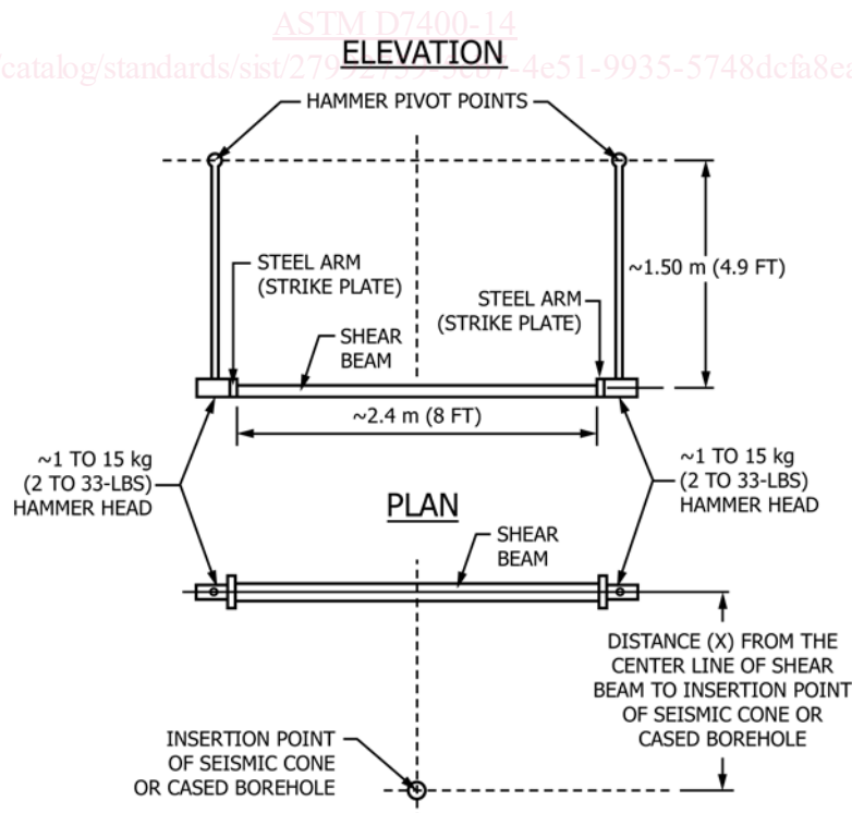
FIG. 1 Typical Downhole Shear Wave Source (Produces SH- Wave Train)
