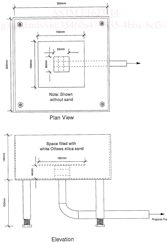
FIG. 9 Sand Burner
