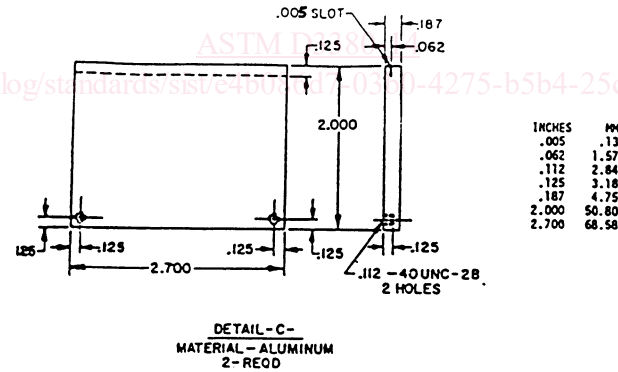
FIG. 6 Test Fixture Construction, Older Design (Fixture B)
