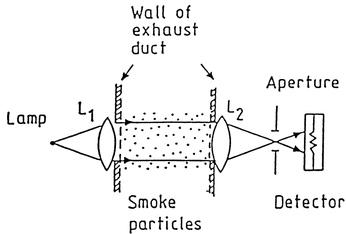
FIG. 3 Optical System
