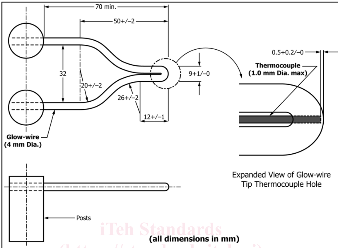
FIG. 1 Glow-Wire and Positioning of Thermocouple
