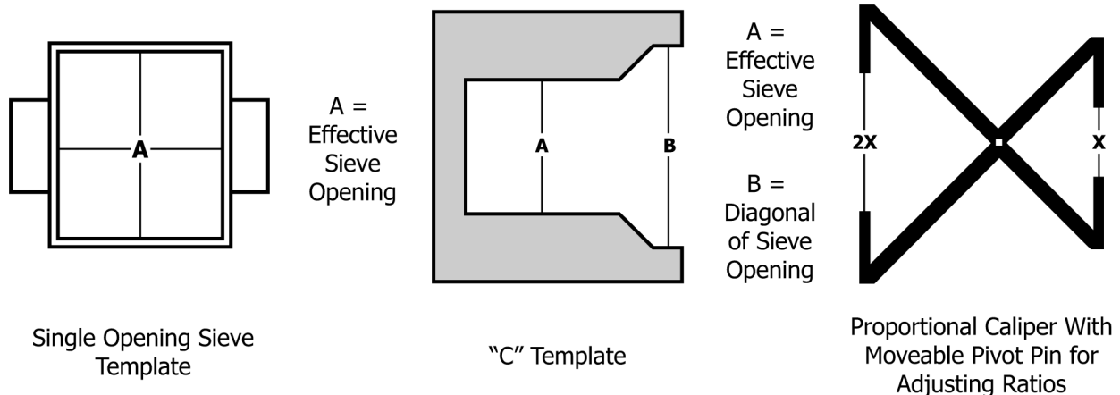
FIG. 1 Single-Opening Sieve Template Riprap Measuring Equipment
