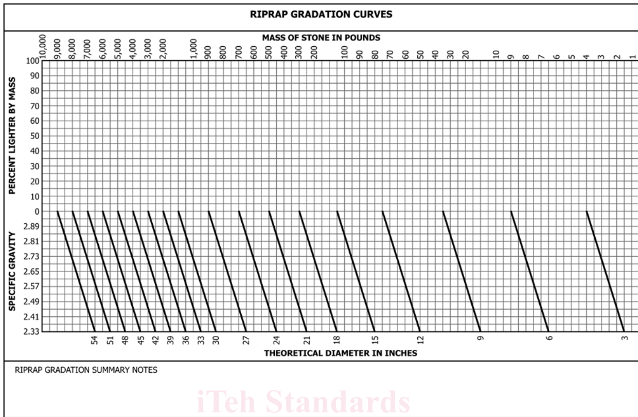
FIG. 2 Typical Grading Graph
